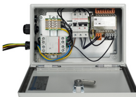
Control box (3*400V / 3*480V)
